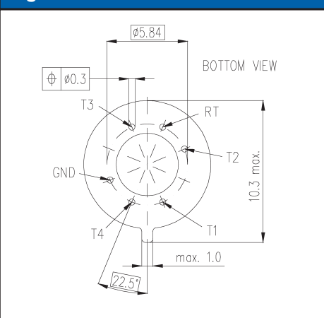
Figure 5. Bottom View
