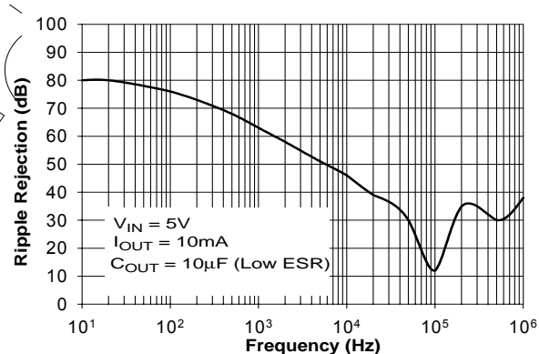
Ripple Rejection vs. Frequency
