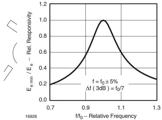
Figure 5. Frequency Dependence of Responsivity
