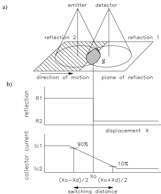
Figure 7. Abrupt reflection change with associated I_c curve
