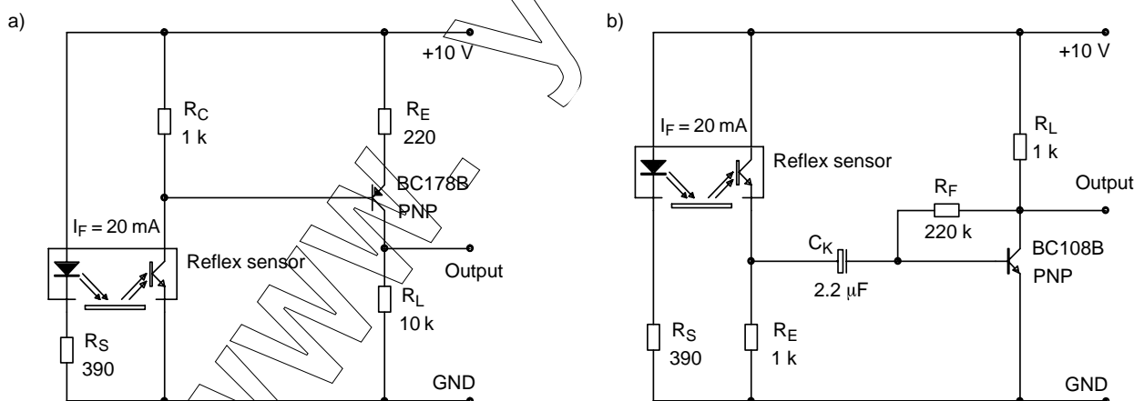
Figure 13. Circuits with transistor amplifier
