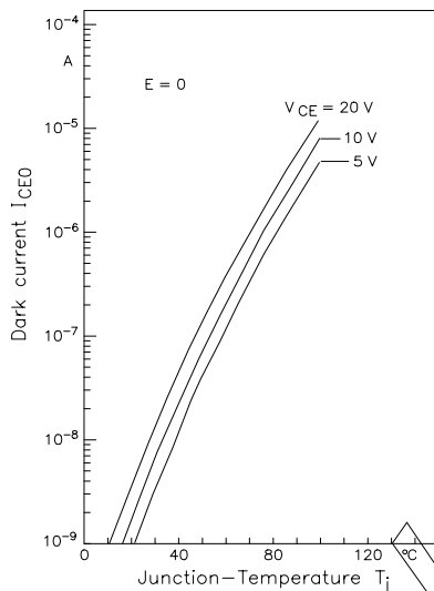
Figure 10. Temperature-dependence of the collector dark current
