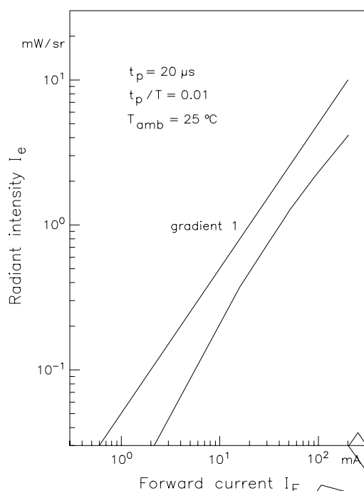
Figure 1. Radiant intensity, I_e = f(I_F) , of the IR transmitter
