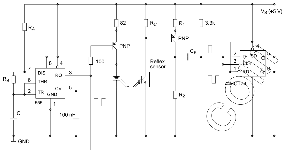
Figure 18. Pulse circuit with buffer storage
