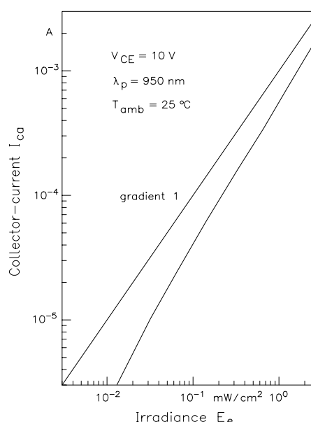
Figure 2. Sensitivity of the reflex sensors' detector
