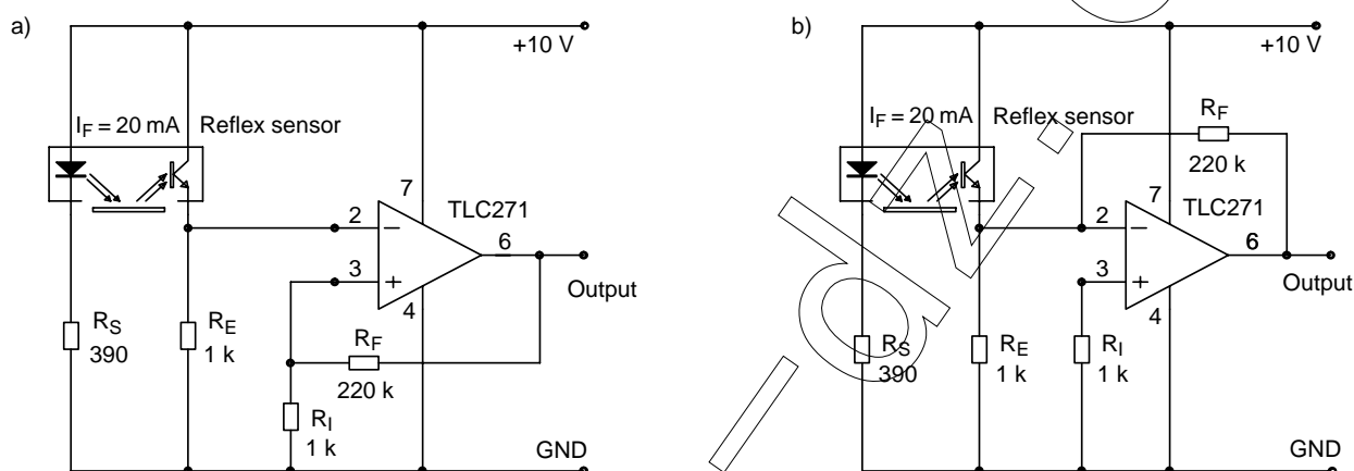
Figure 12. Circuits with operational amplifier
