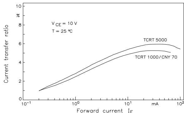
Figure 3. Coupling factor k = f(I_F) of the reflex sensors
