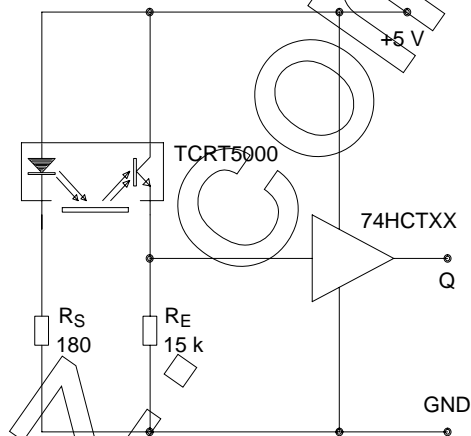
Figure 11. Reflex sensor - basic circuit
