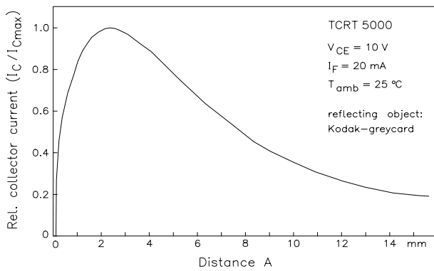
a) TCRT5000
