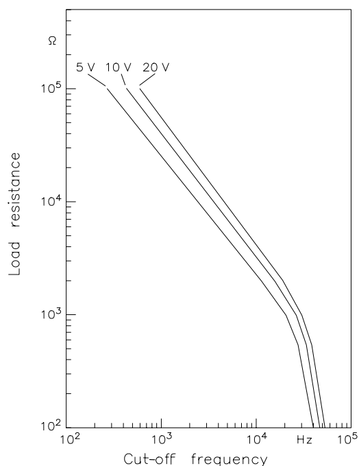
Figure 5. Cut-off frequency, f_c
