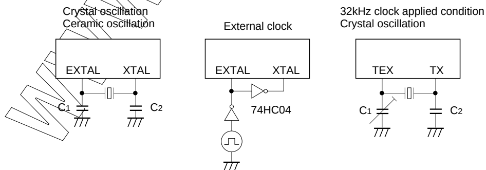
Fig. 2. Clock applied condition
