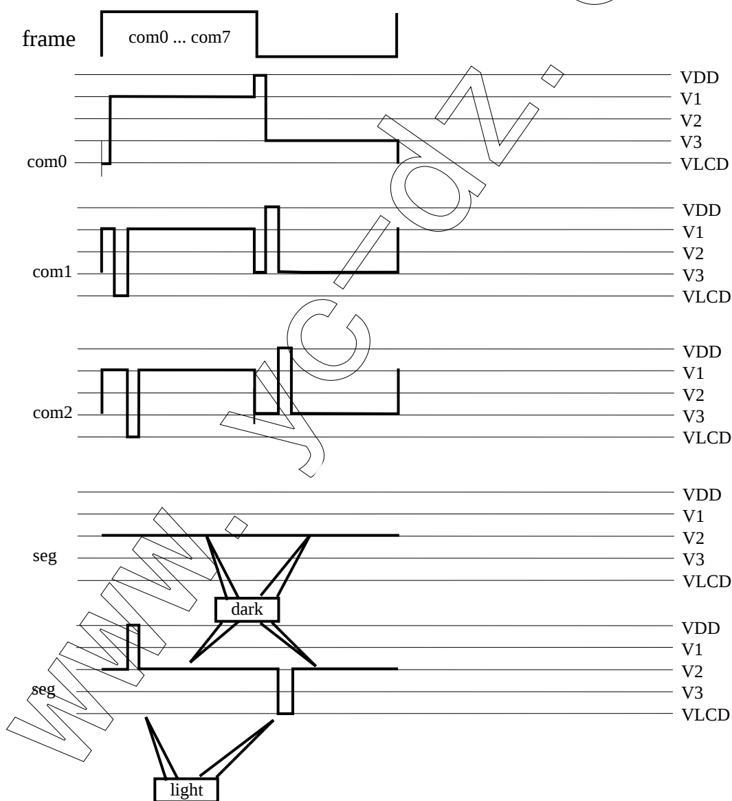
Fig.14 Lcd wave 1/4 bias, 1/8 duty
