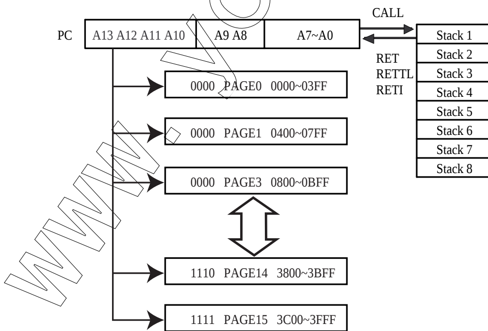
Fig.4 Program counter organization
