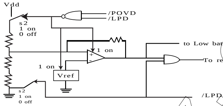
Fig6. The relation between /LPD,/POVD
