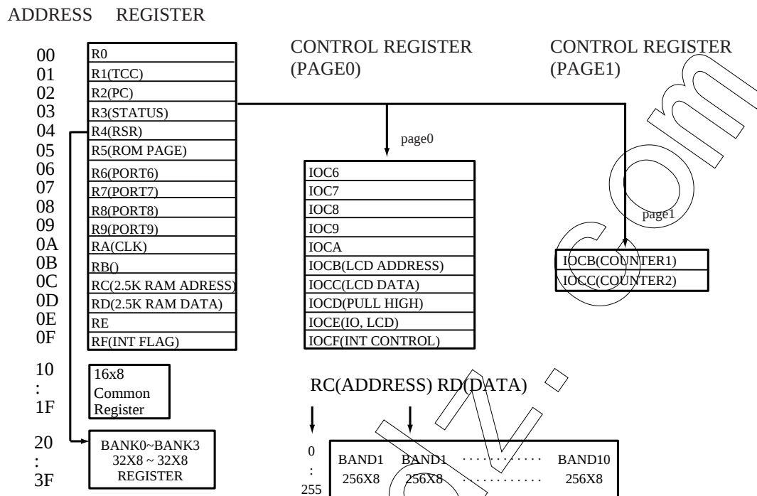
Fig.5 Data memory configuration
