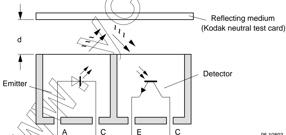
Figure 1. Test circuit
