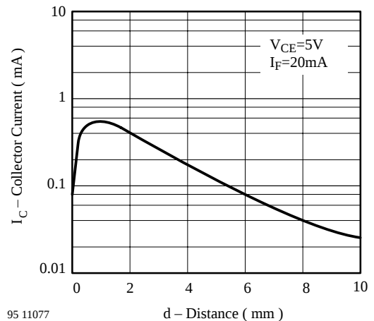
Figure 7. Collector Current vs. Distance
