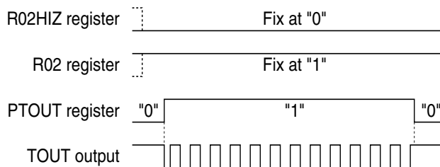
Fig. 4.10.6.3 Output waveform of the TOUT signal
