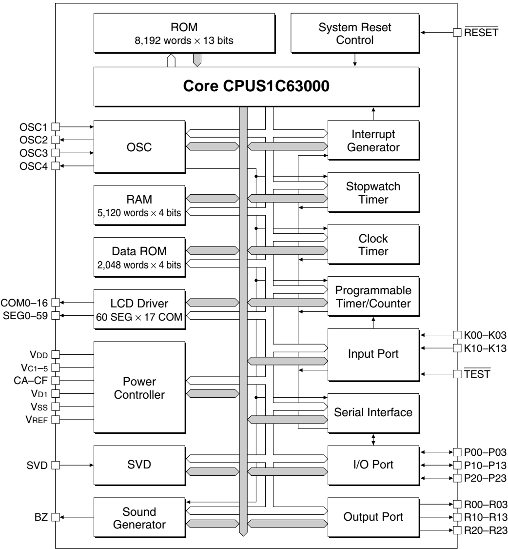
Fig. 1.2.1 Block diagram
