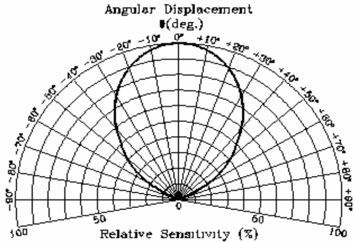
Sensitivity Diagram
