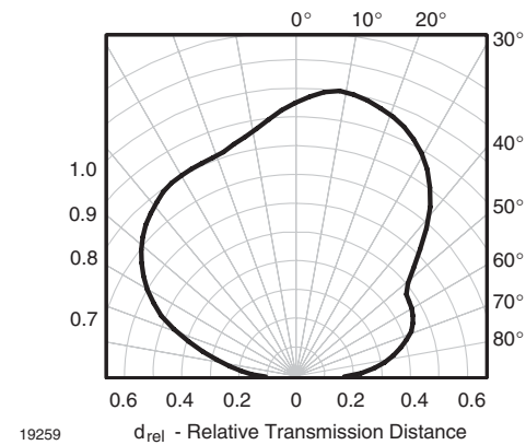
Figure 12. Vertical Directivity \phi_y
