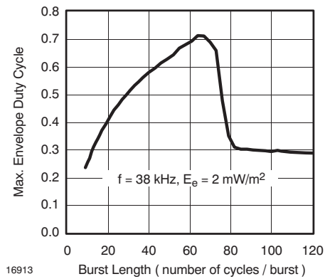
Figure 8. Max. Envelope Duty Cycle vs. Burstlength
