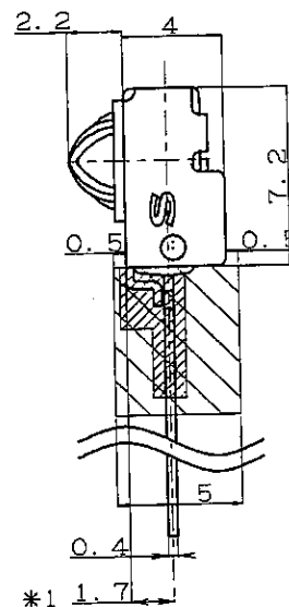
Example of mounting drawing from solder side (Reference)
