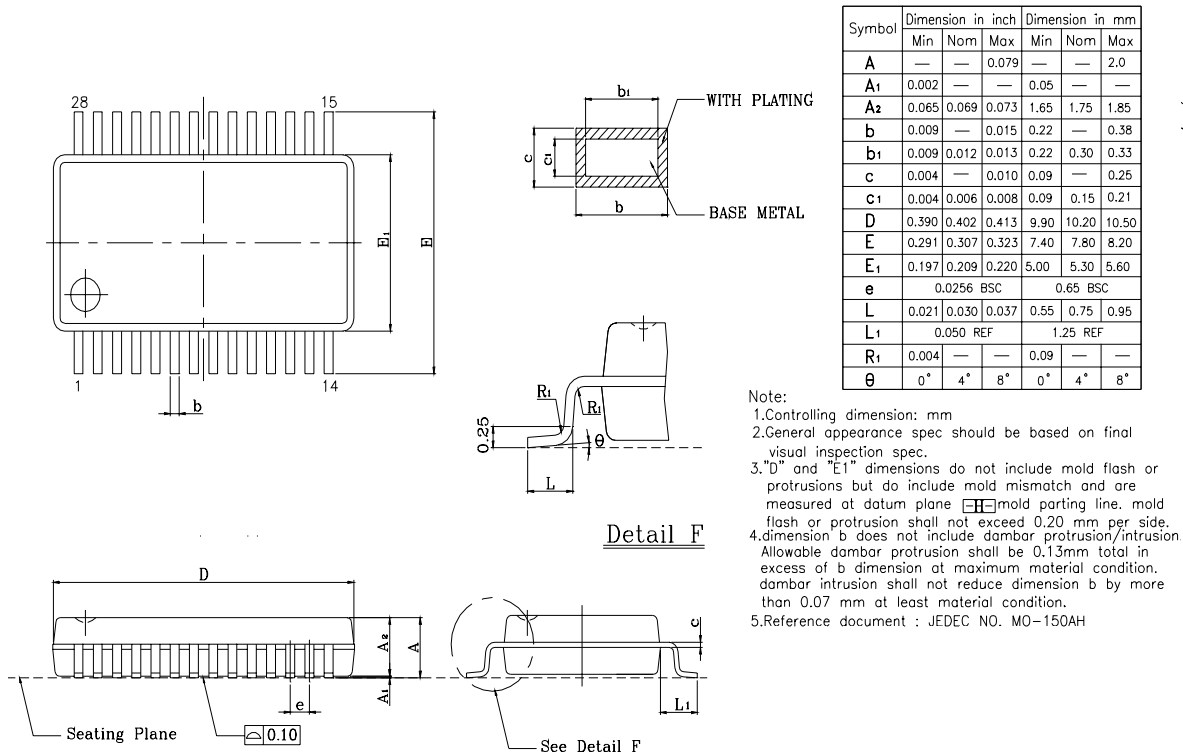
Figure 10. 28-Pin SSOP Package Drawing
