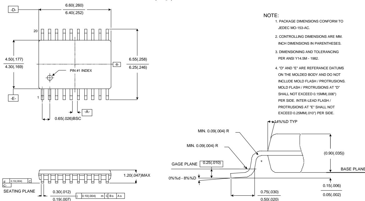
Figure 11. 20-Pin TSSOP Package Drawing
