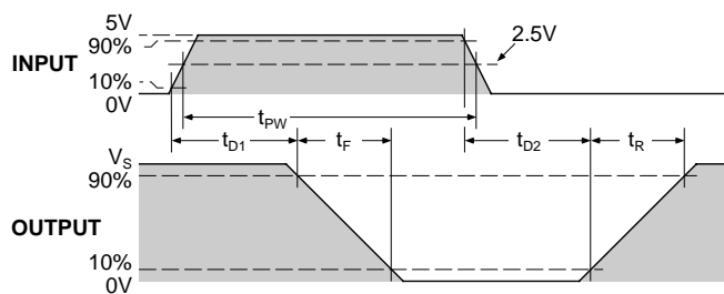
Figure 1b. Inverting Timing
