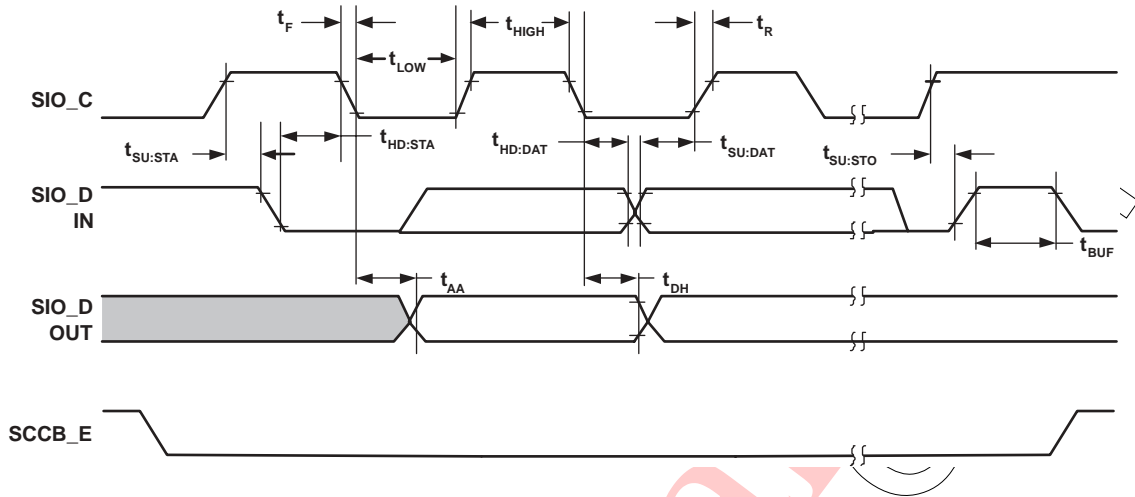
Figure 4 SCCB Timing Diagram
