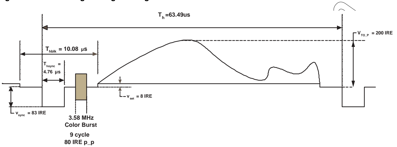
(A) HORIZONTAL TIMING FOR NTSC
