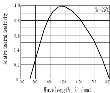
Fig.5 Spectral Sensitivity
