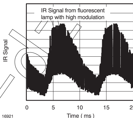
Figure 15. IR Signal from Fluorescent Lamp with high Modulation
