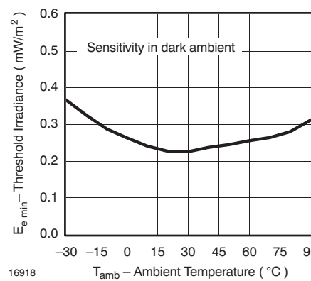
Figure 10. Sensitivity vs. Ambient Temperature
