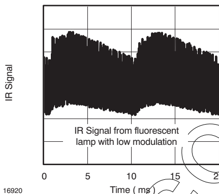
Figure 14. IR Signal from Fluorescent Lamp with low Modulation
