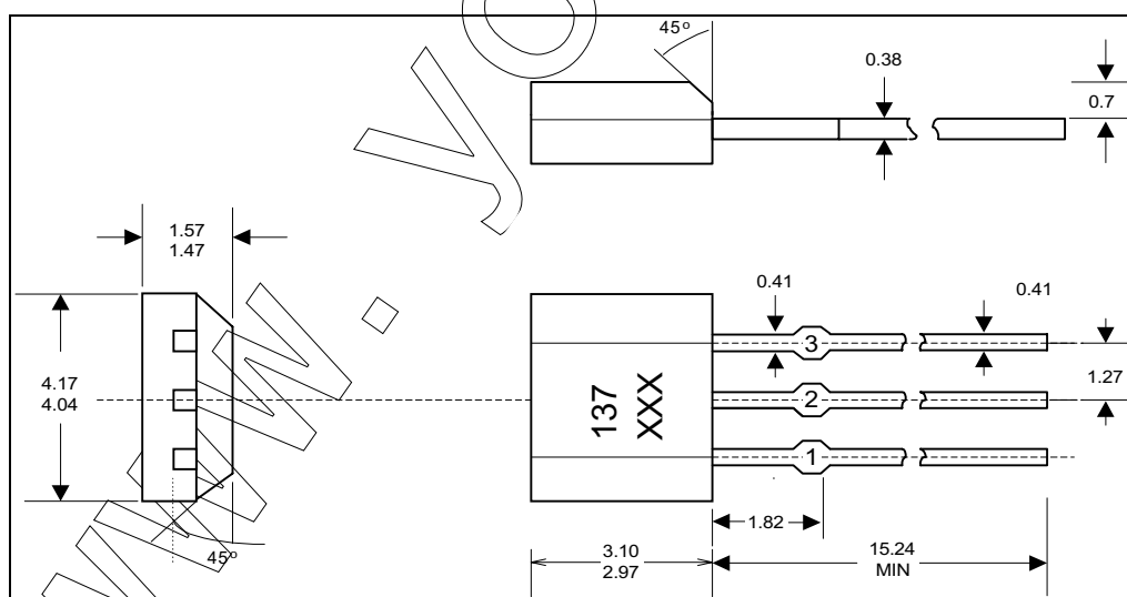
Package Dimension
