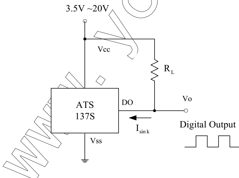
Fig.2 Application circuit
