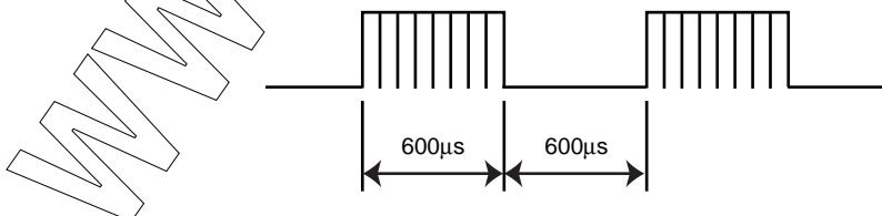
Fig.1 Transmit signal.
