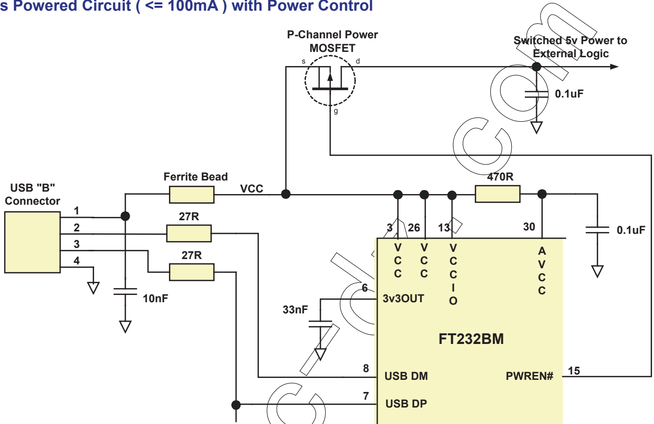
Figure 16 Bus Powered Circuit ( \leq 100\text{mA} ) with Power Control
