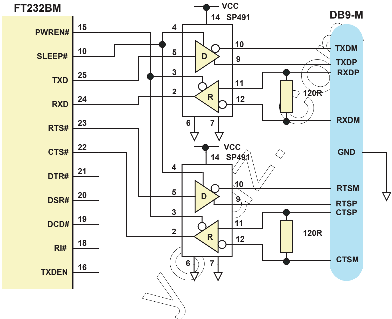
Figure 11 USB => RS422 Converter Configuration
