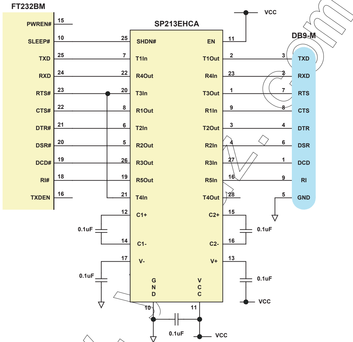
Figure 10 USB => RS232 Converter Configuration
