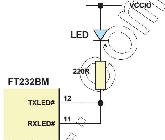
Figure 14 Single LED Configuration
