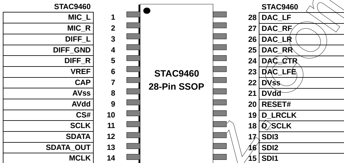
Figure 9. STAC9460 Pin Designation
