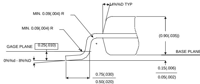
Figure 11. 20-Pin TSSOP Package Drawing
