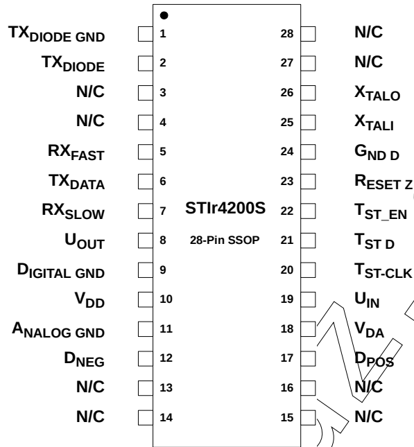
Figure 8. STIr4200S 28-Pin SSOP Pin Assignment Drawing
