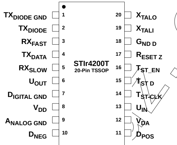
Figure 9. STIr4200T 20-Pin TSSOP Pin Assignment Drawing
