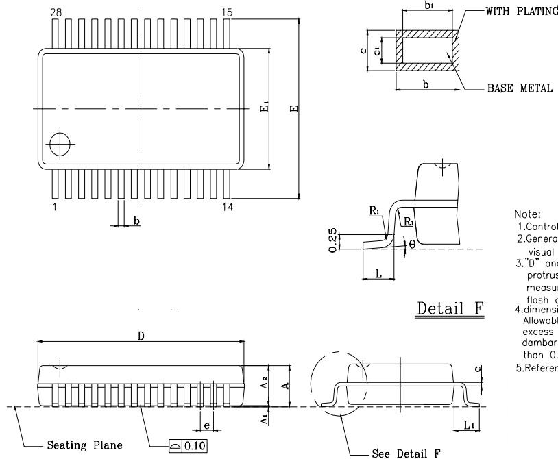
Figure 10. 28-Pin SSOP Package Drawing
