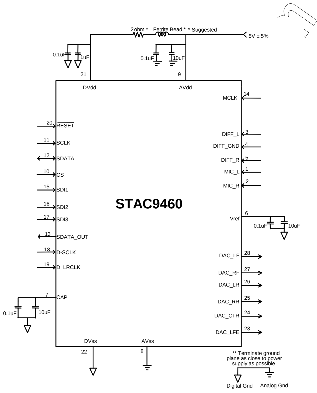
Figure 2. Typical Connection Diagram
