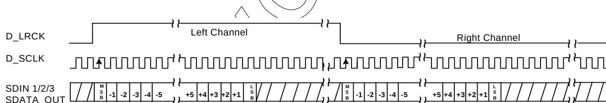
Figure 5. I 2 S Left Justified Format
