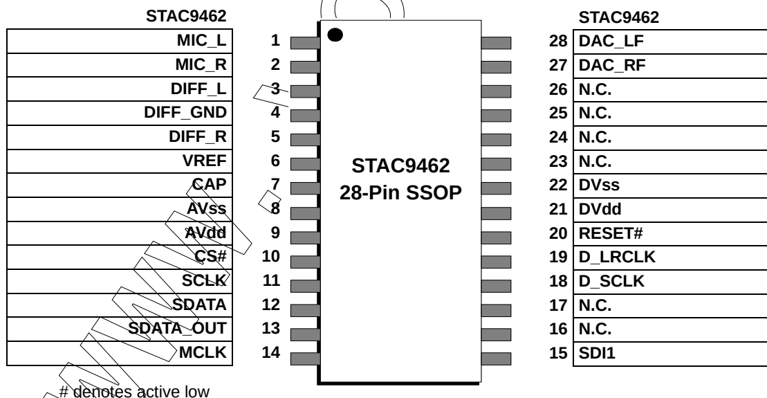
Figure 10. STAC9462 Pin Designation
