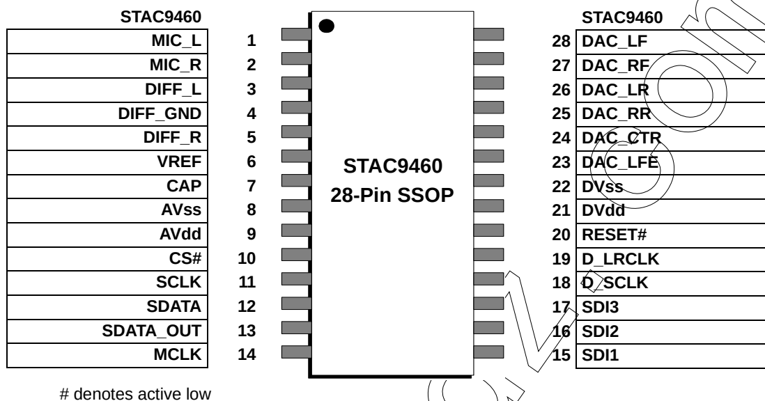
Figure 9. STAC9460 Pin Designation
