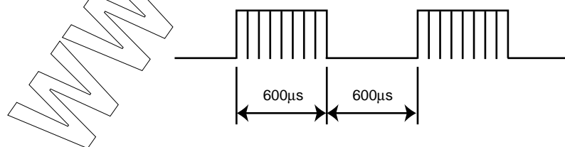
Carrier frequency=f o , Duty=50%
