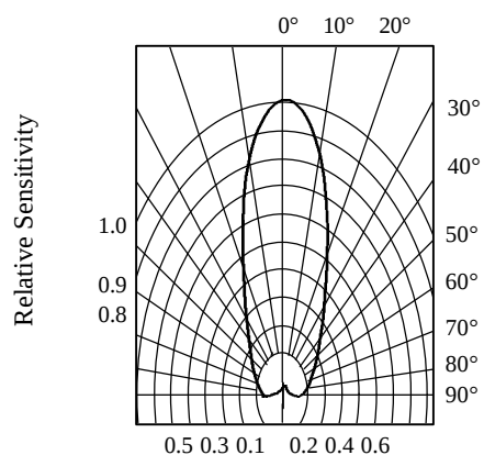
FIG.7 SENSITIVITY DIAGRAM
