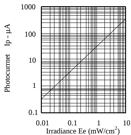
FIG.6 PHOTOCURRENT VS. IRRADIANCE = 850 nm
