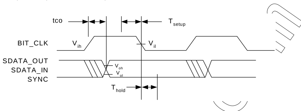
Figure 5. Data Setup and Hold Timing
