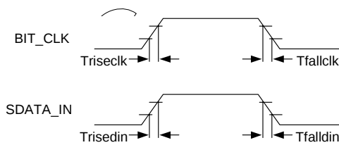
Figure 6. Signal Rise and Fall Times Timing
