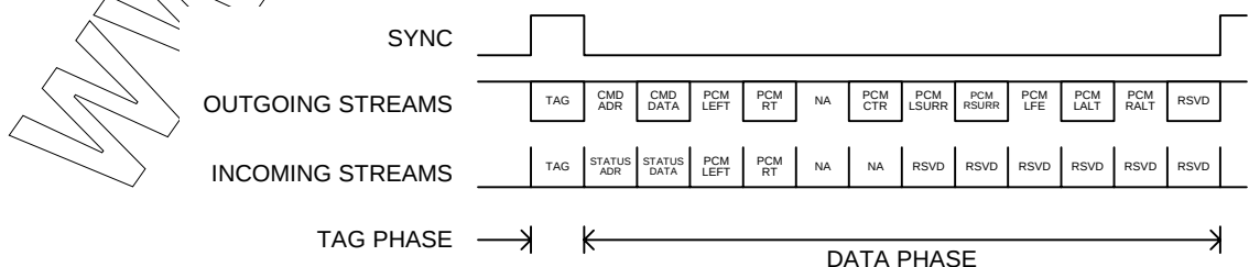
Figure 11. AC'97 Standard Bi-directional Audio Frame
