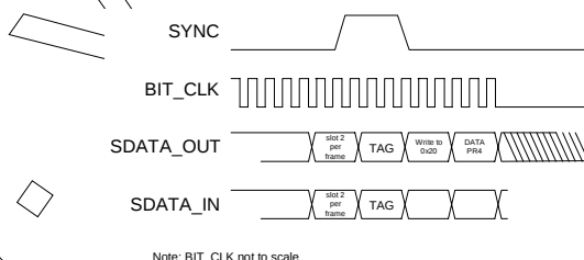
Figure 16. STAC9750/51 Powerdown Timing
