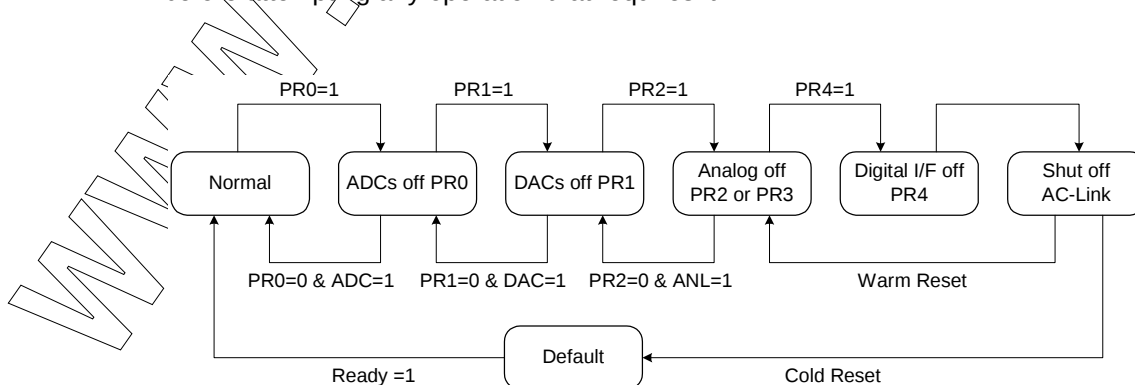
Figure 19. Example of STAC9750/51 Powerdown/Powerup flow
