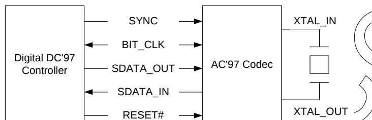
Figure 10. AC-Link to its Companion Controller
