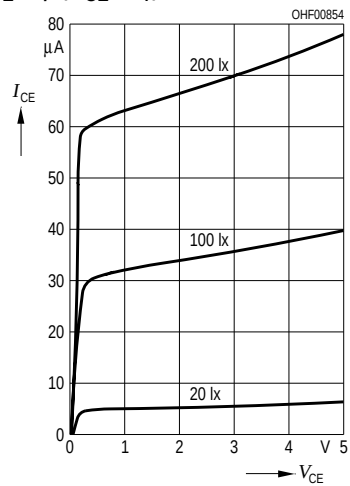
Collector-Emitter Current I_{\text{CE}} = f(V_{\text{CE}}, E_V)
