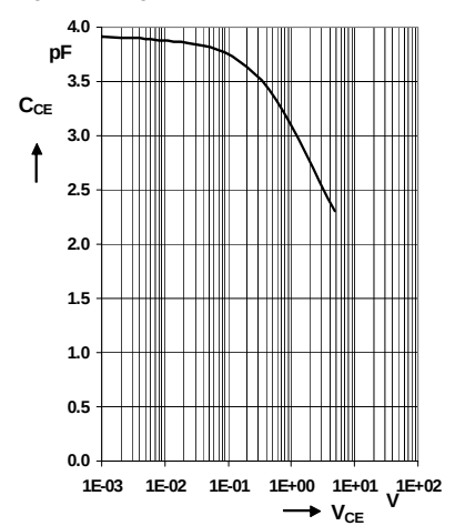
Collector-Emitter Capacitance C_{\text{CE}} = f(V_{\text{CE}})
