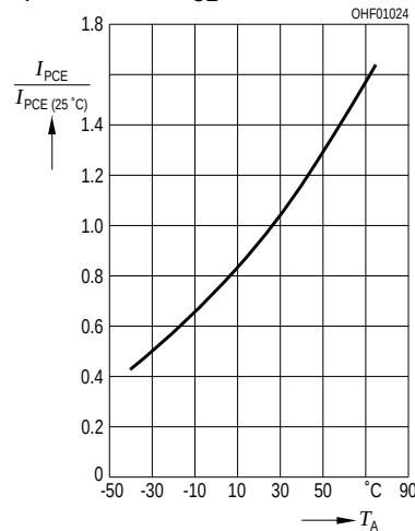
Photocurrent I_{\text{PCE}}/I_{\text{PCE}(25^\circ\text{C})} = f(T_A) E_V = 1000 \text{ lx}, V_{\text{CE}} = 1 \text{ V} \dots 5 \text{ V}
