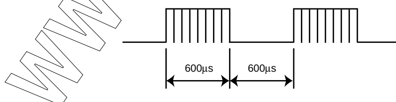
Fig.1 Transmit signal
