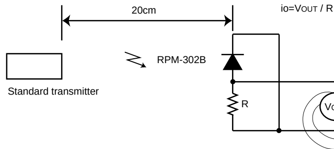
Fig.2 Measurement of standard transmitter proofreading
