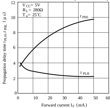
Fig.10-b Propagation Delay Time vs. Forward Current
