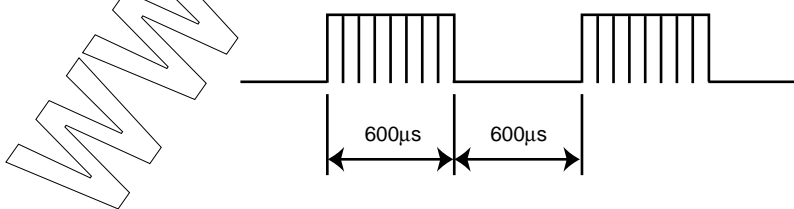
Fig.1 Transmit signal
