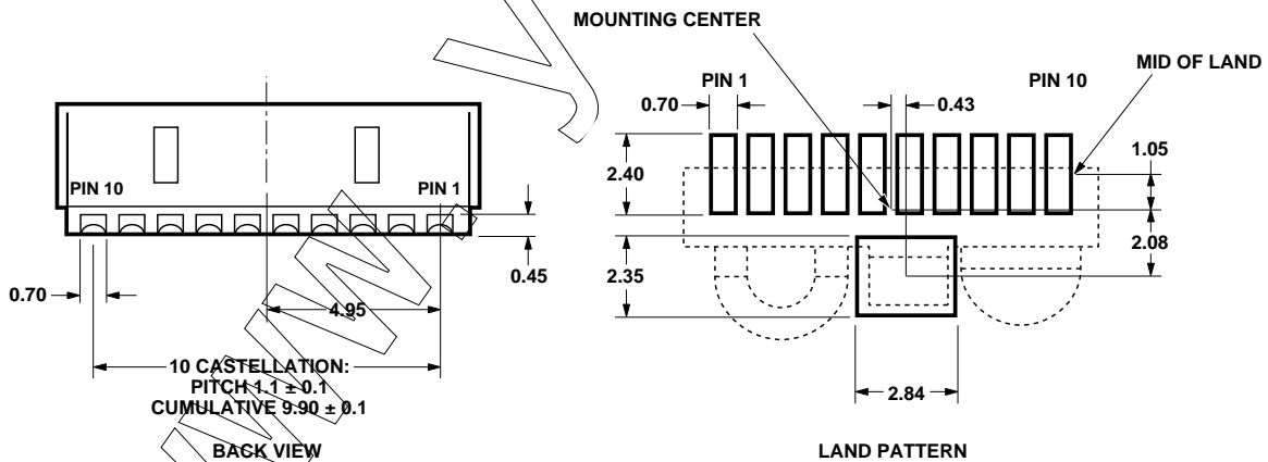
BACK VIEW
