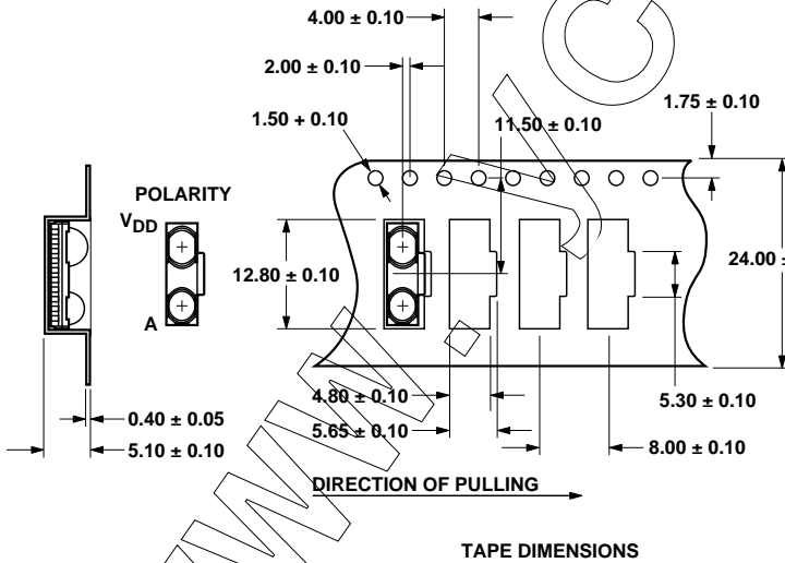
TAPE DIMENSIONS
