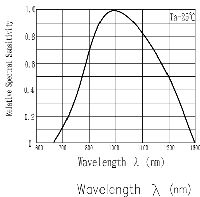
Fig.5 Spectral Sensitivity
