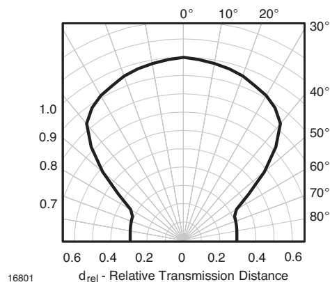
Figure 12. Directivity
