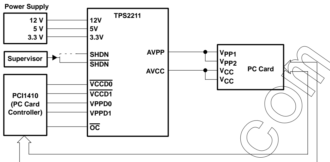
Figure 3-4. TPS2211 Typical Application
