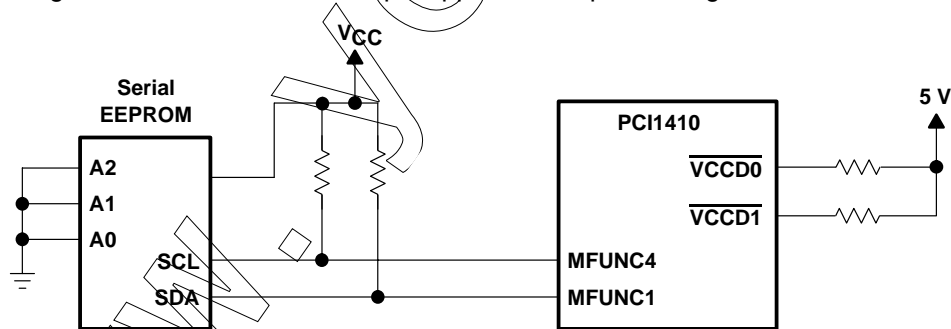
Figure 3–9. Serial EEPROM Application
