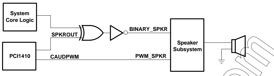
Figure 3-7. Sample Application of SPKROUT and CAUDPWM
