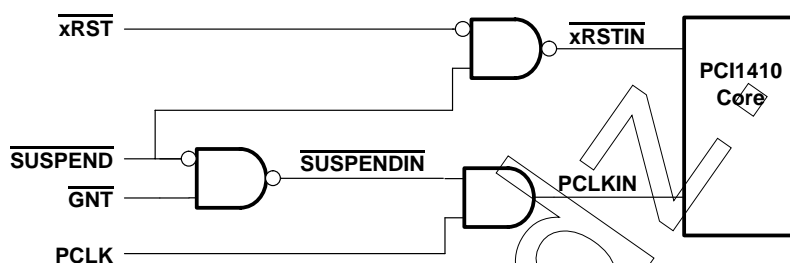
Figure 3–17. Suspend Logic Diagram
