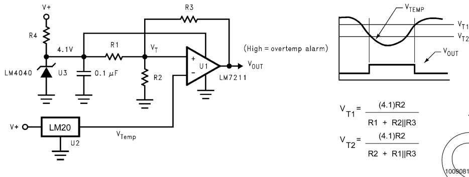
FIGURE 6. Centigrade Thermostat
