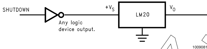
FIGURE 7. Conserving Power Dissipation with Shutdown
