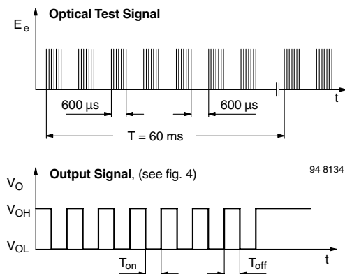
Figure 3. Output Function
