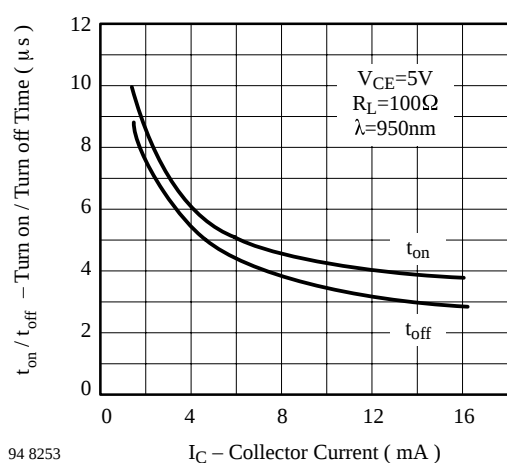
Figure 9. Turn On/Off Time vs. Collector Current
