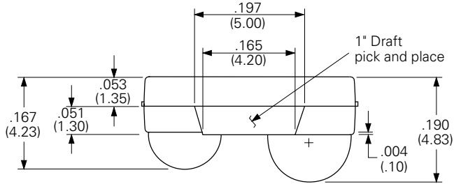
Figure 24. IRMS6400/IRMT6400 detail drawings with optional side view or top view mounting
