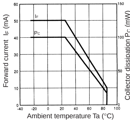
Forward Current vs. Collector Dissipation Temperature Rating
