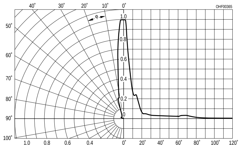
Radiation characteristics I_{\text{rel}} = f(\varphi) , SFH 4592
