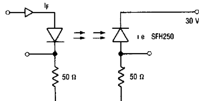
SFH450V/451V/750V Test Circuit for Switching Times
