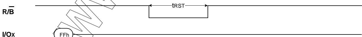
Figure 15. RESET Operation
