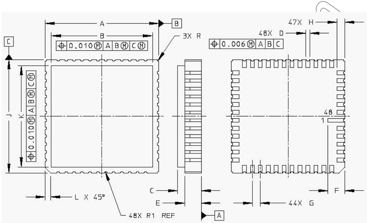
Figure 21. 48 Terminal ceramic leadless chip carrier (bottom view)
