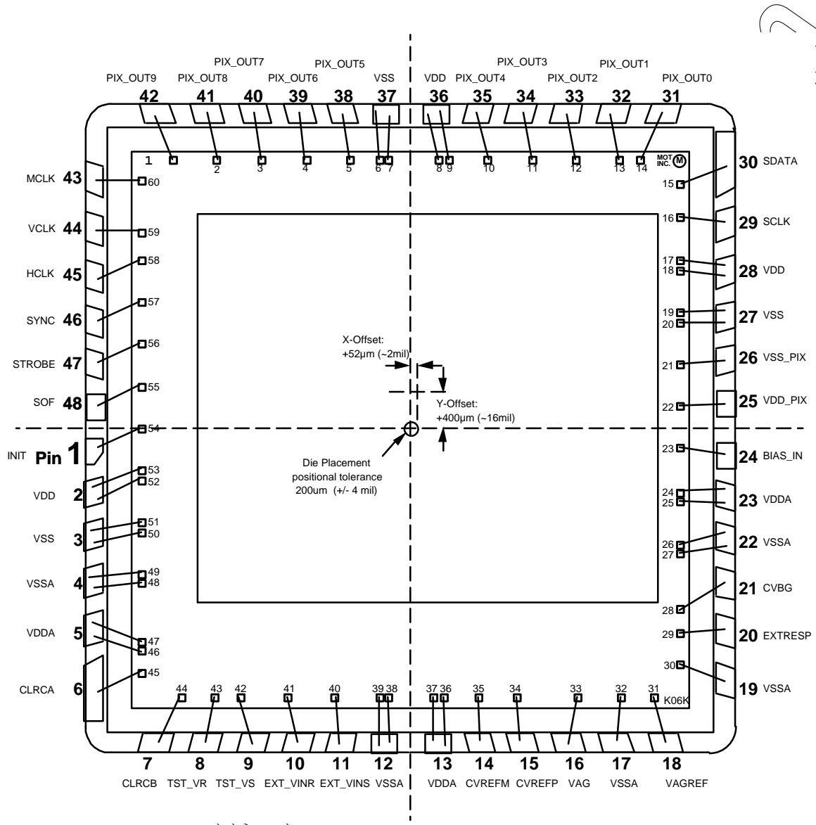
Figure 23. Center of the focal plane array with respect to the die cavity (top view)
