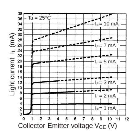
Light Current vs. Collector-Emitter Voltage Characteristics (Typical)
