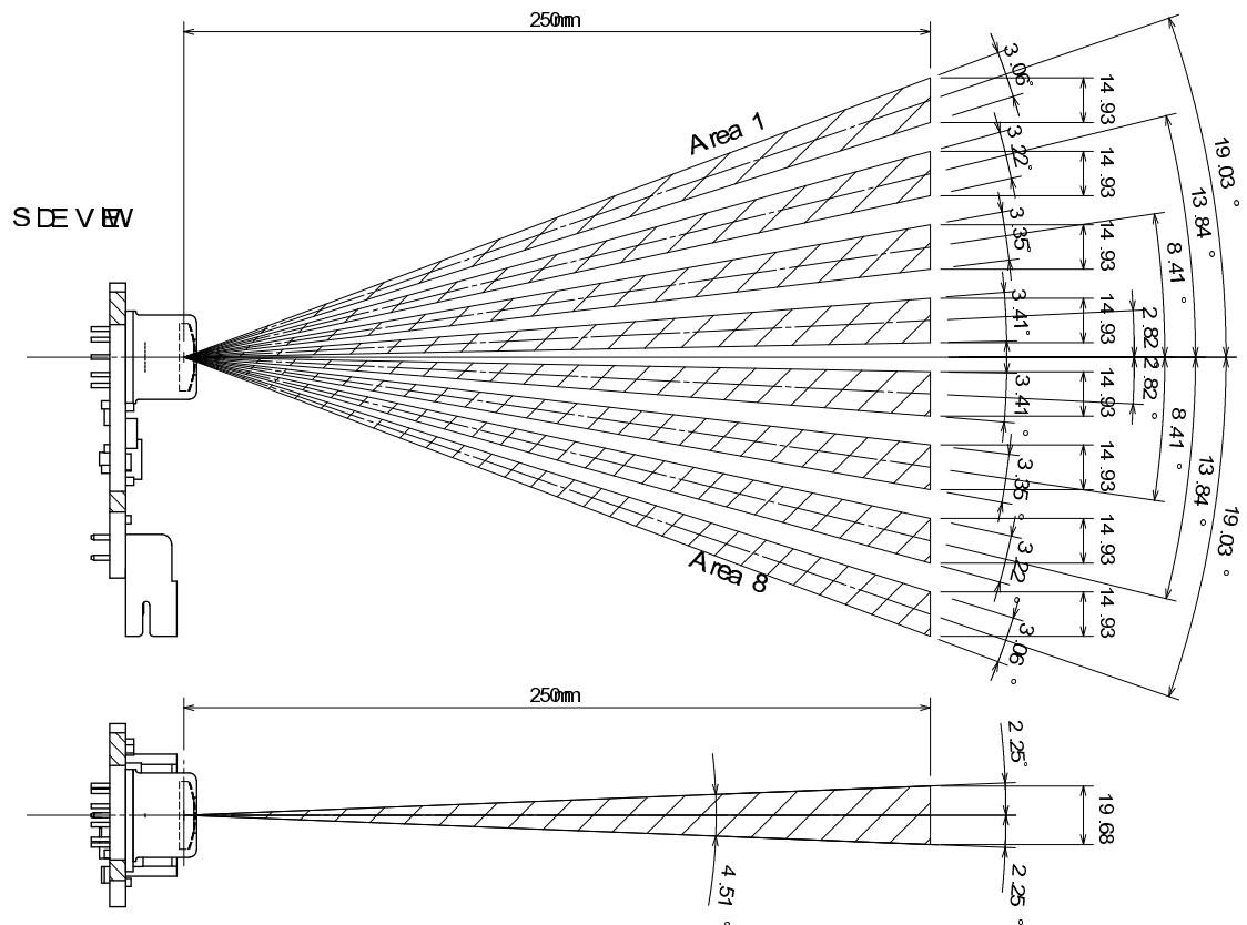
Fig. 3 : Detection Area
