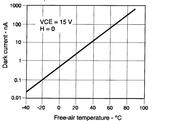
Fig. 3 Dark Current vs Temperature
