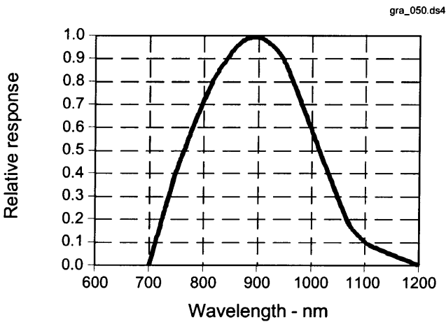
Fig. 5 Spectral Responsivity
