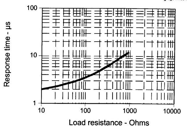
Fig. 4 Non-Saturated Switching Time vs Load Resistance
