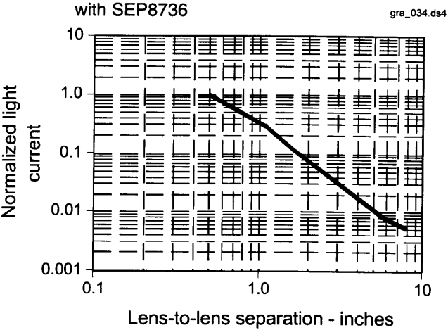
Fig. 6 Coupling Characteristics with SEP8736
