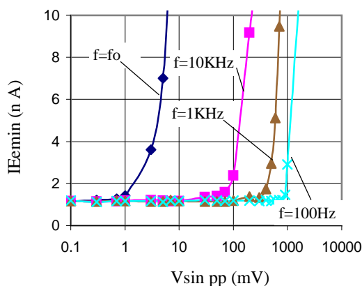
SENSITIVITY vs SUPPLY VOLTAGE DISTURBANCES
