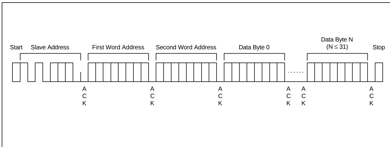
Figure 4-11. Page Write Operation
