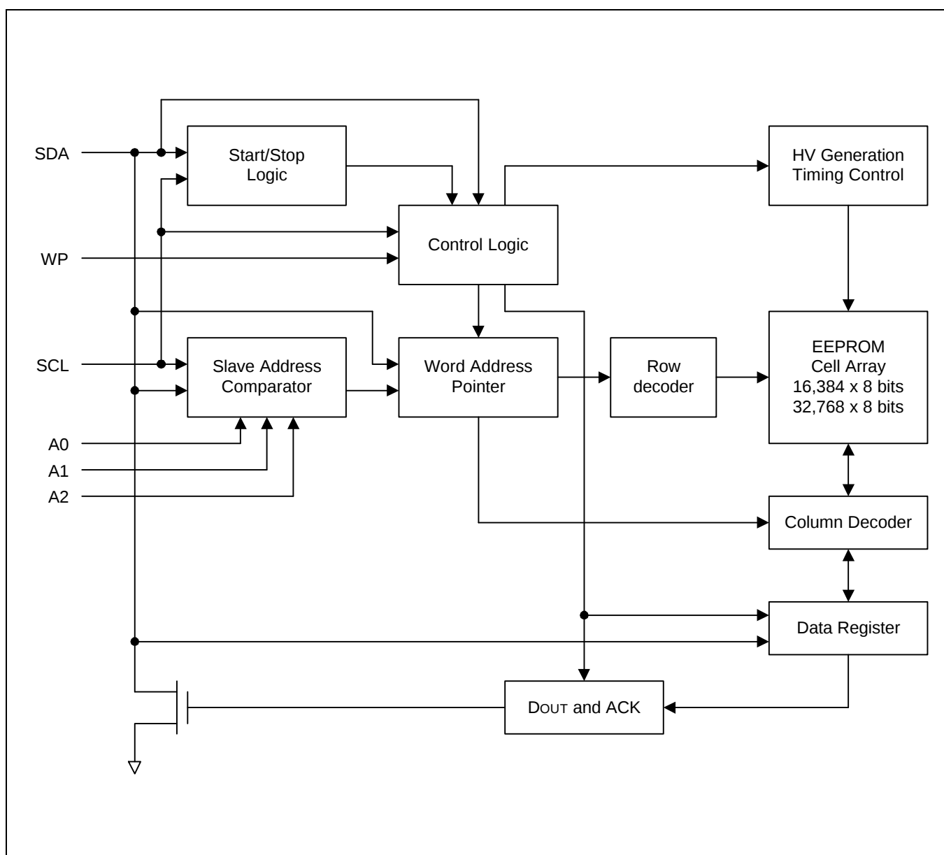
Figure 5-1. S524AD0XD1/D0XF1 Block Diagram
