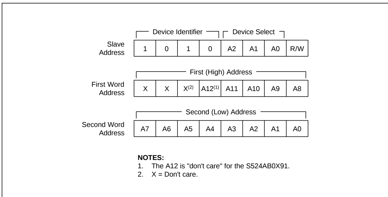
Figure 4-9. Device Address
