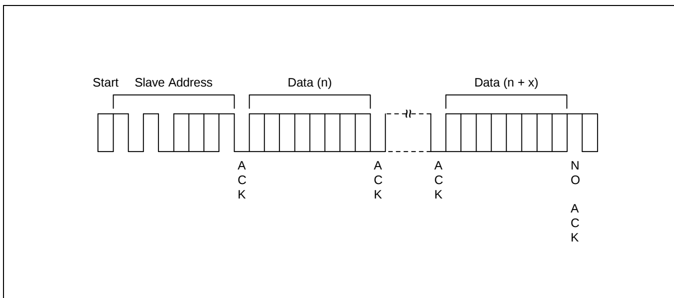
Figure 2-15. Sequential Read Operation
