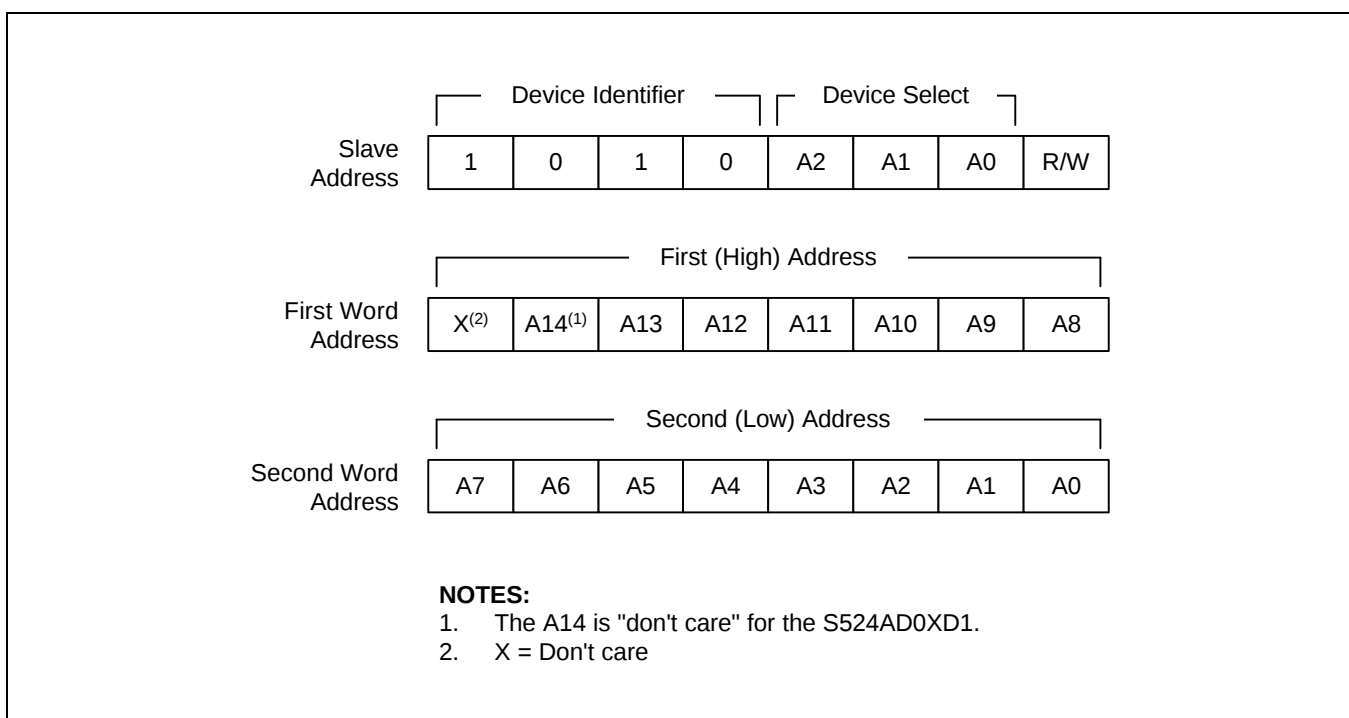
Figure 5-9. Device Address
