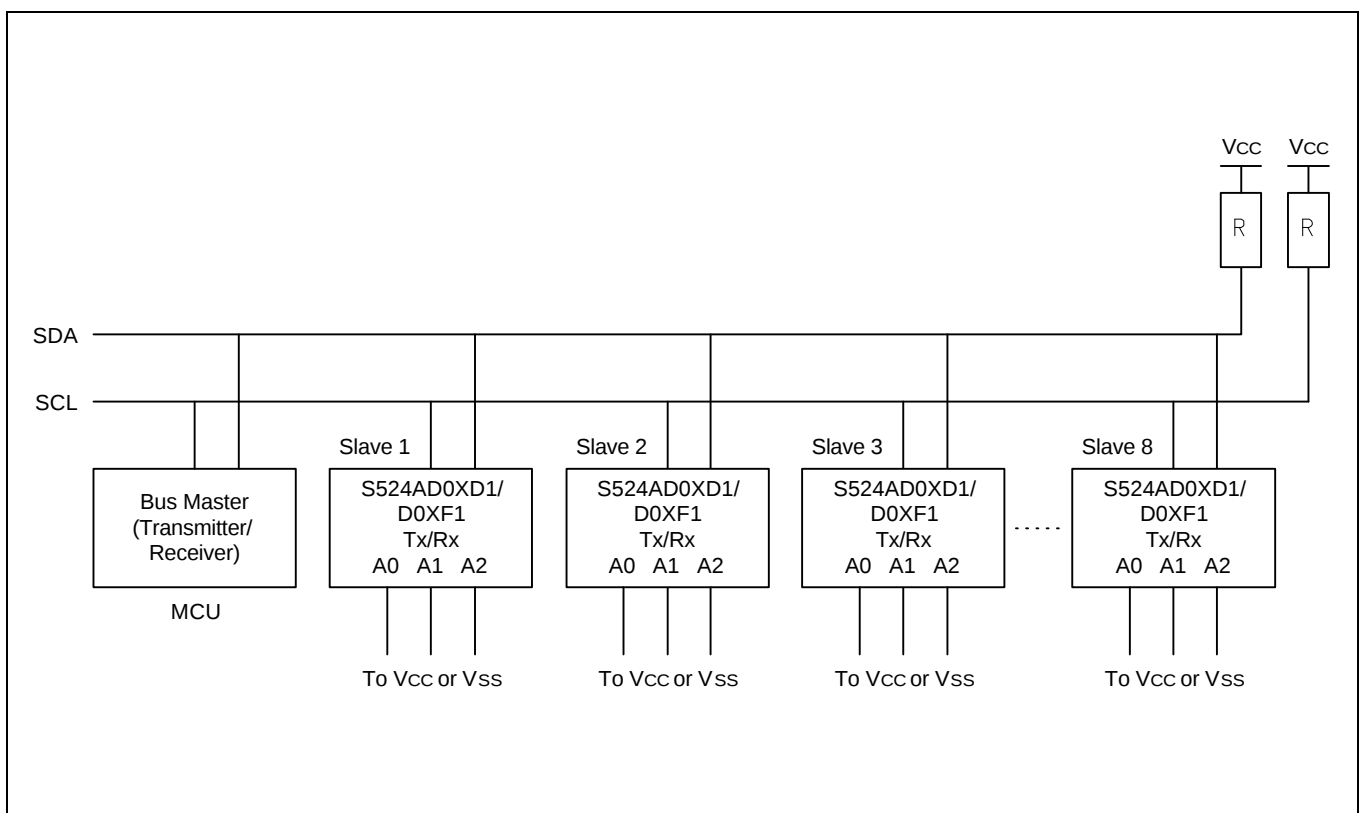
Figure 5-6. Typical Configuration
