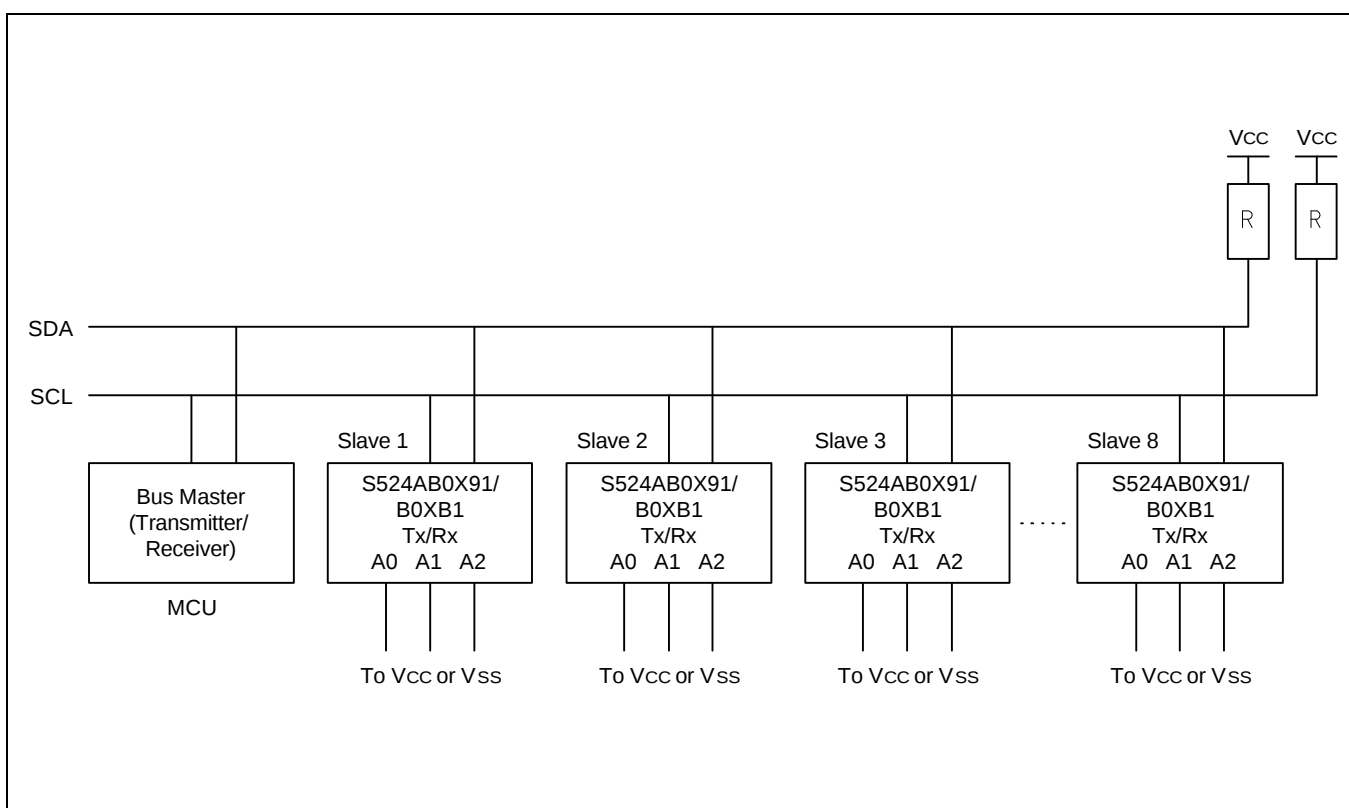
Figure 4-6. Typical Configuration
