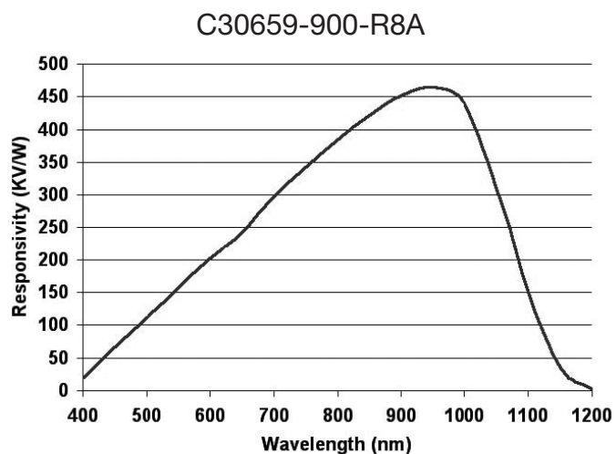
Figure 2. Spectral Responsivity
