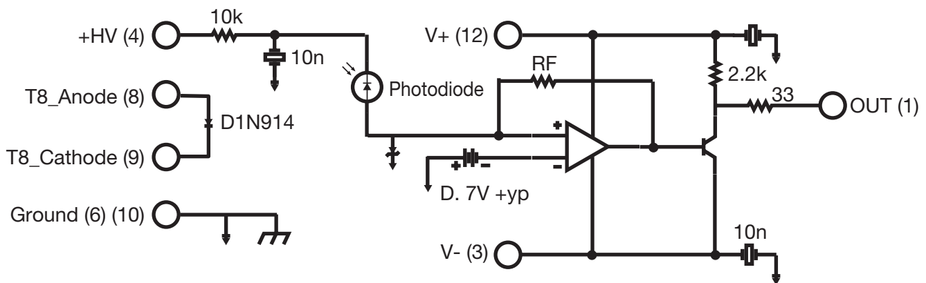
Figure 1. C30659 Series Block Diagram
