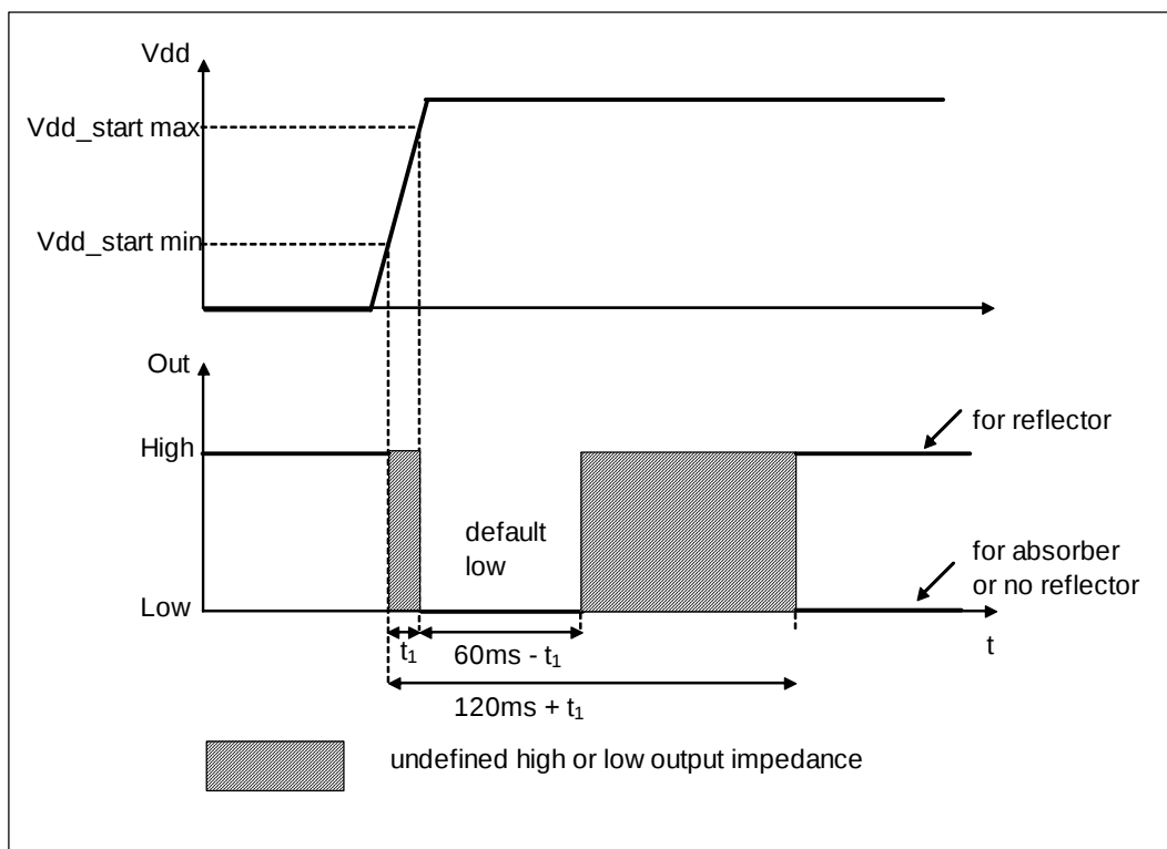
Figure 2 Startverhalten Start-up sequence
