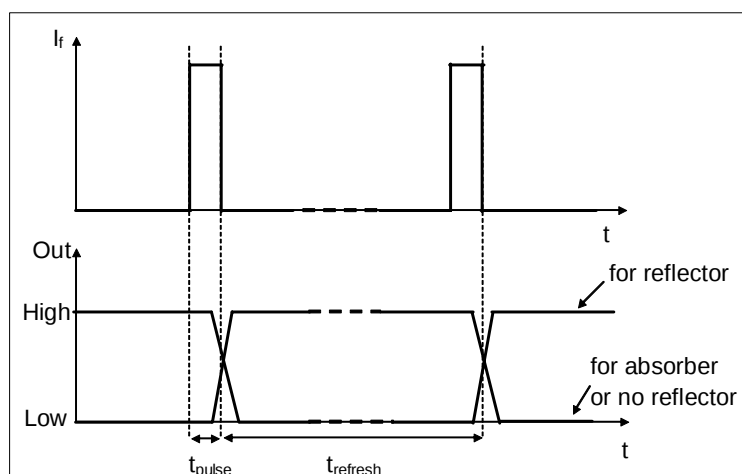
Figure 3 Timing diagram
